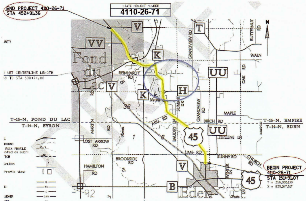
Figure 6: USH 45 Re-Surfacing Project
