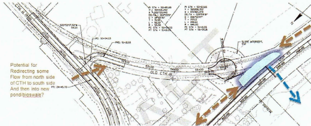
Figure 11: Potential Stormwater Facility, USH 45/Old CTH H
